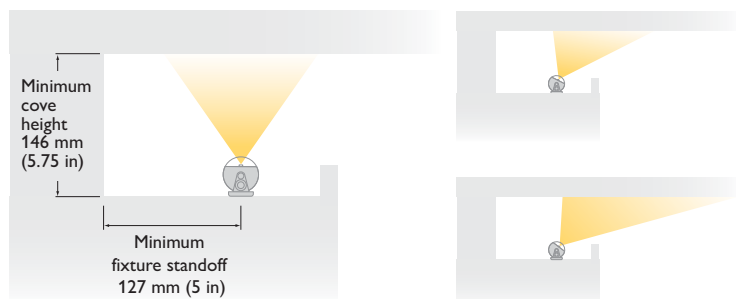
eW Cove QLX Powercore 180° rotation
