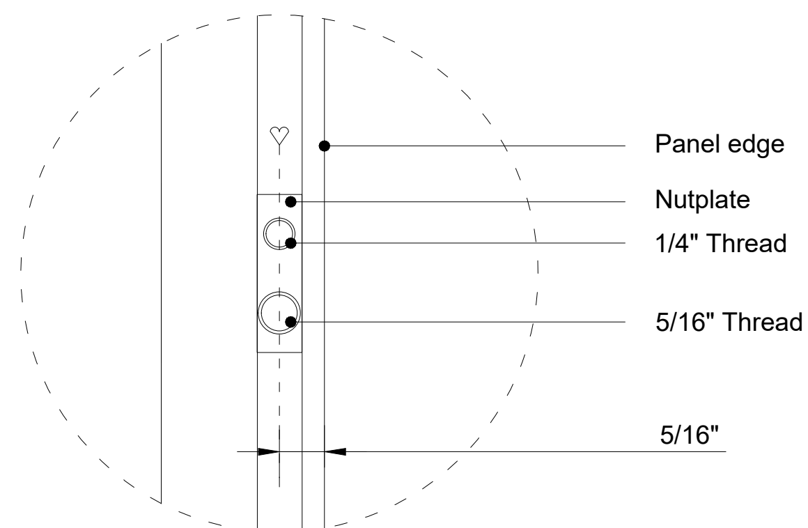
Detail 1 (1:1)
