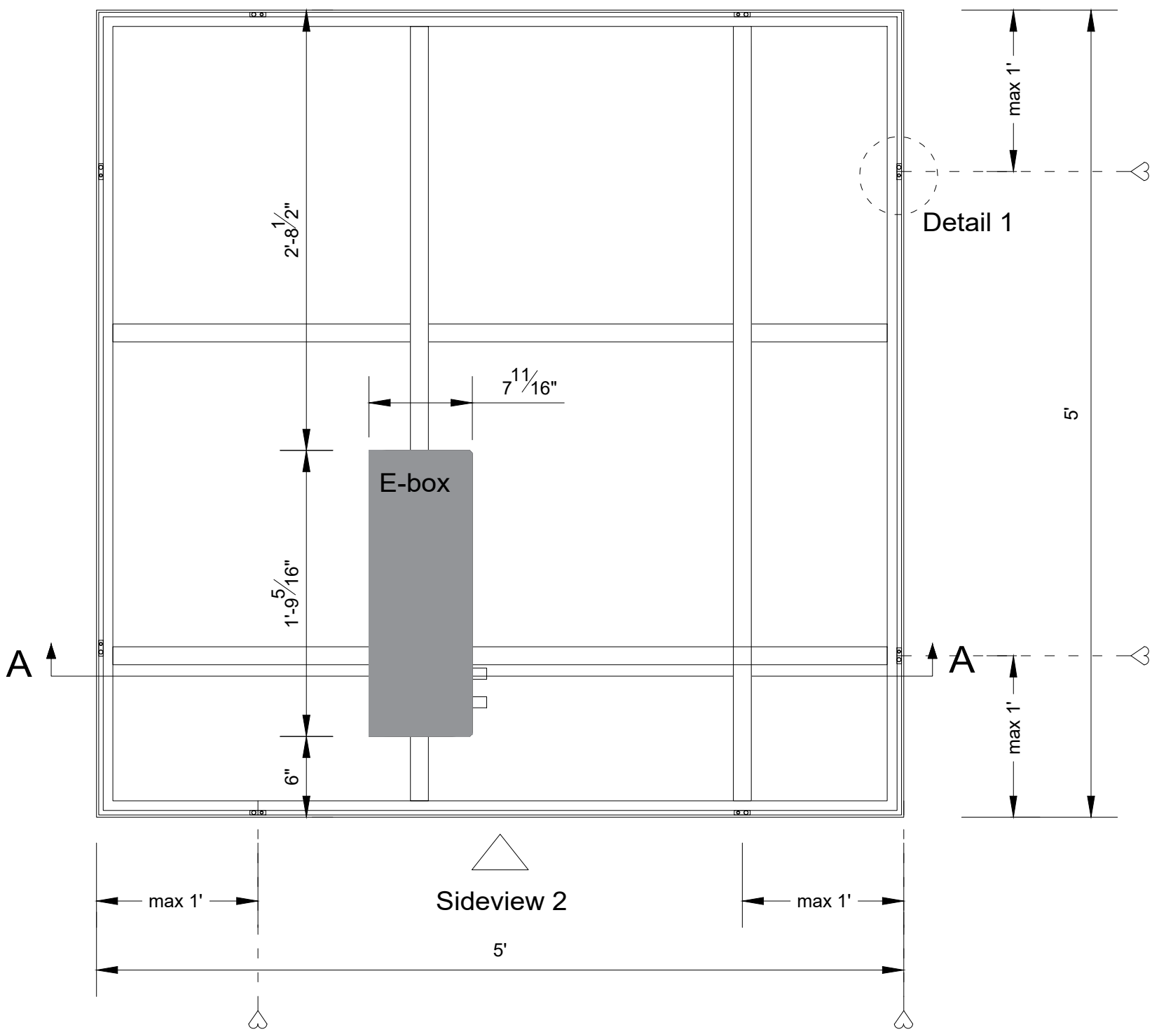
Sideview 2 - mounting position (1:10)
