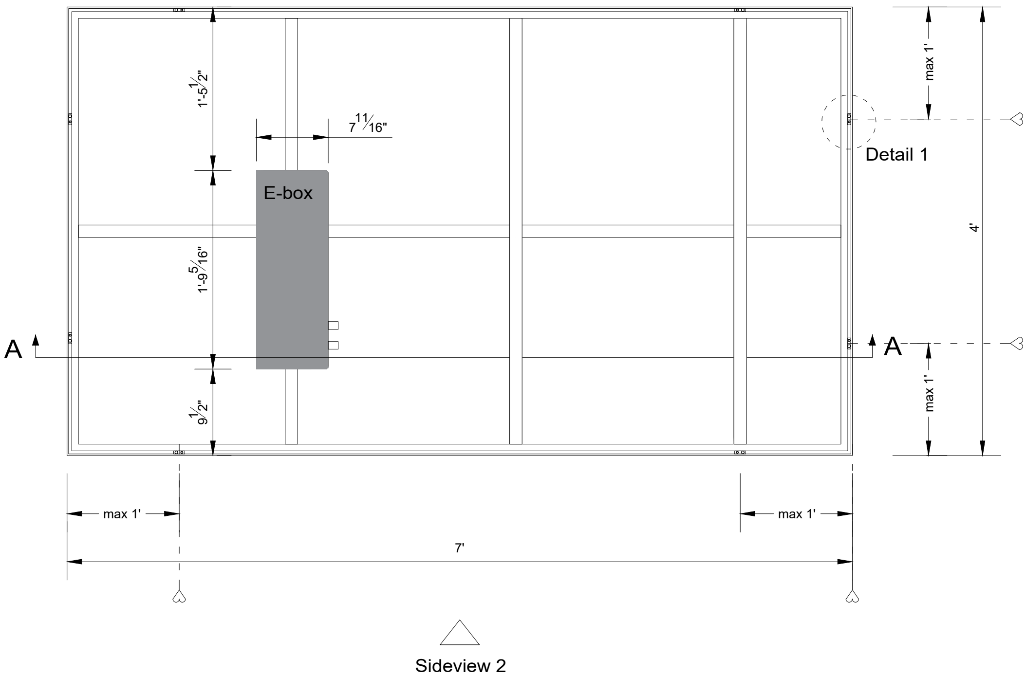
Backview (1:10)
