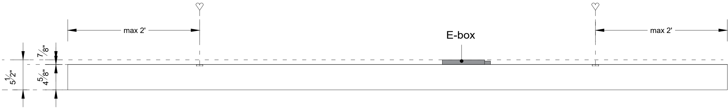
Sideview 2 - mounting position (1:10)
