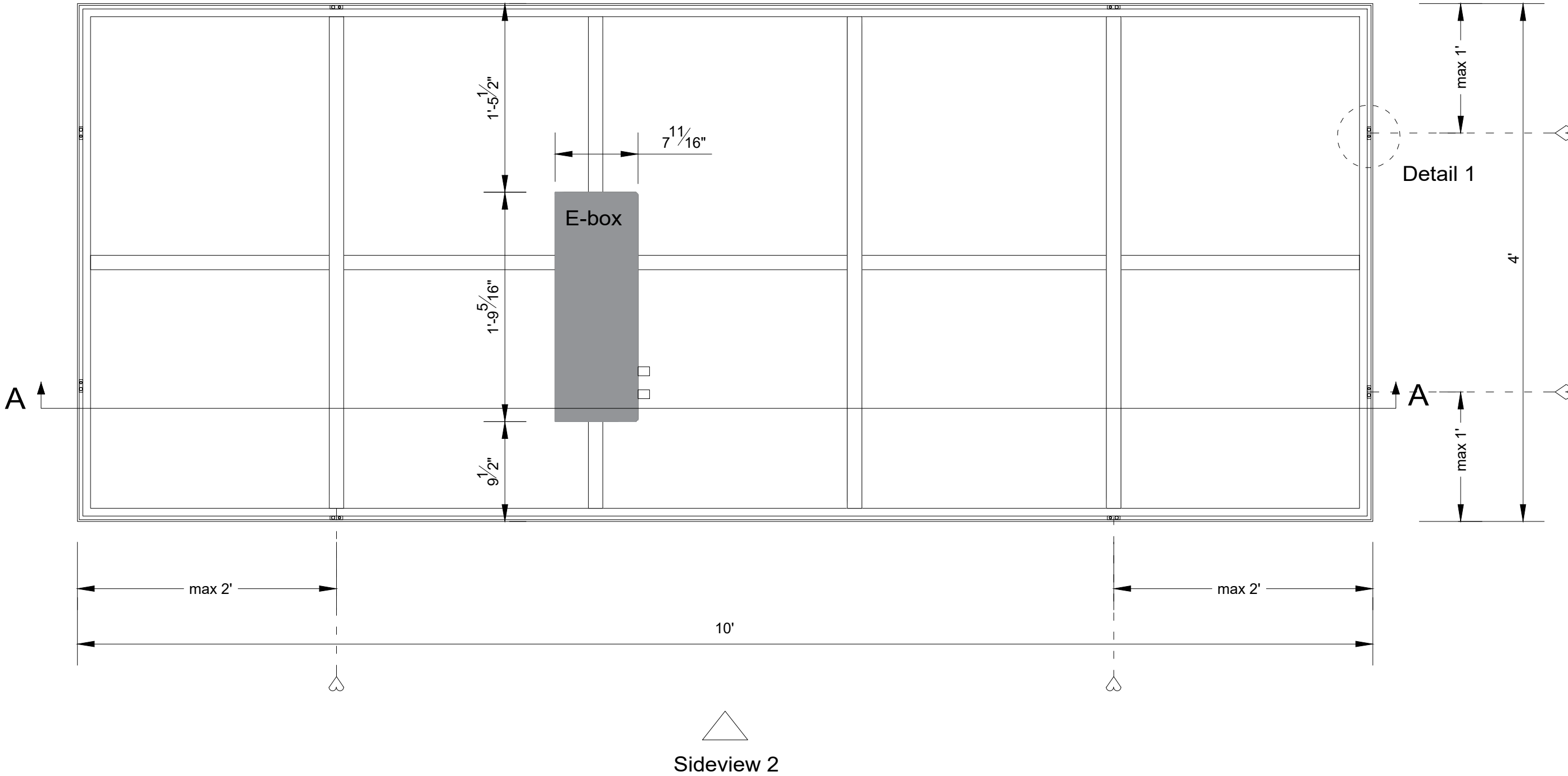
Backview (1:10)
