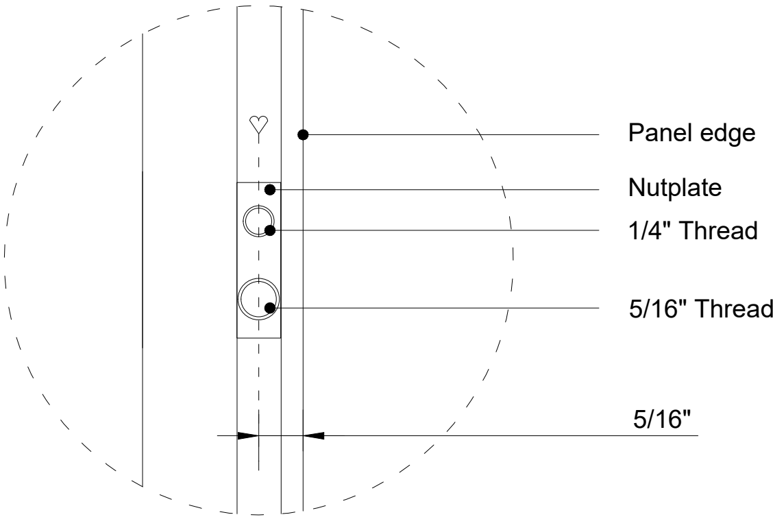
Detail 1 (1:1)
