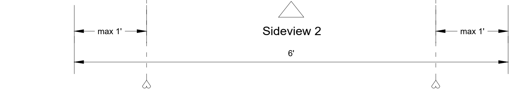
Sideview 2 - mounting position (1:10)
