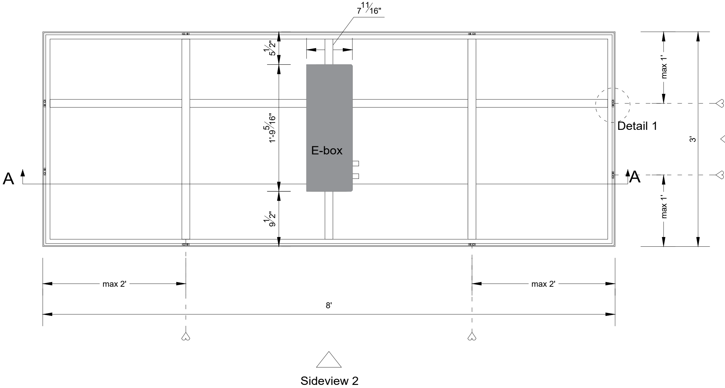
Backview (1:10)
