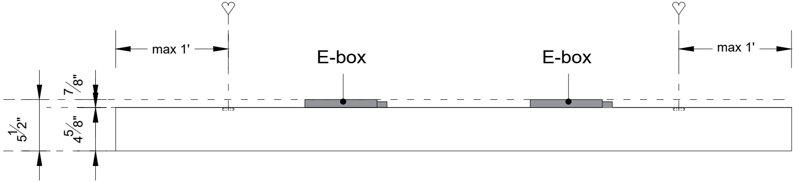
Sideview 2 - mounting position (1:10)
