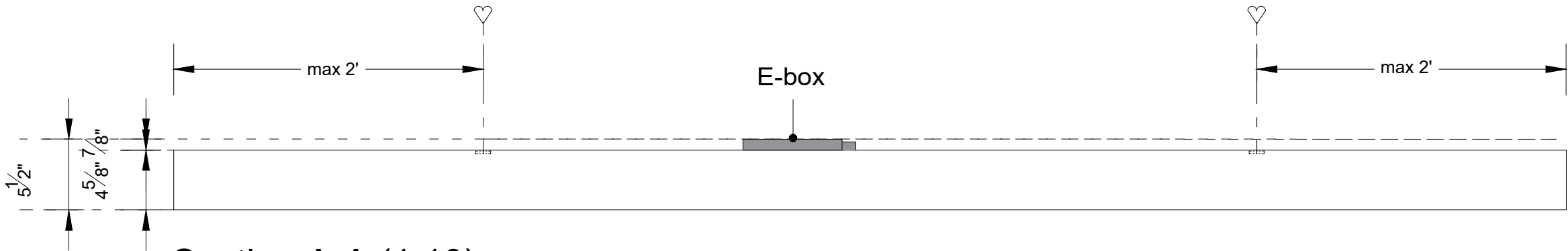
Section A-A (1:10)
