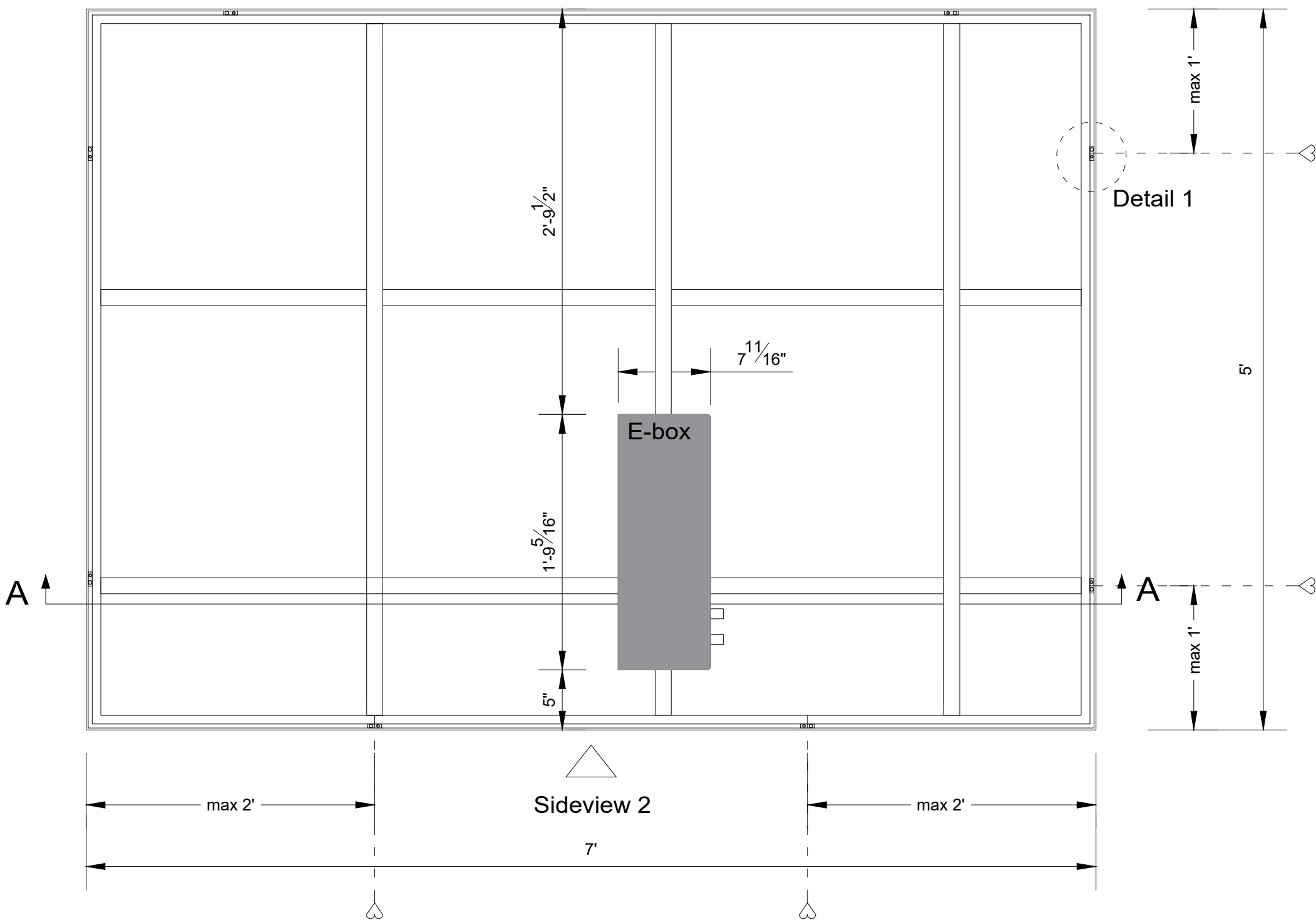
Sideview 2 - mounting position (1:10)
