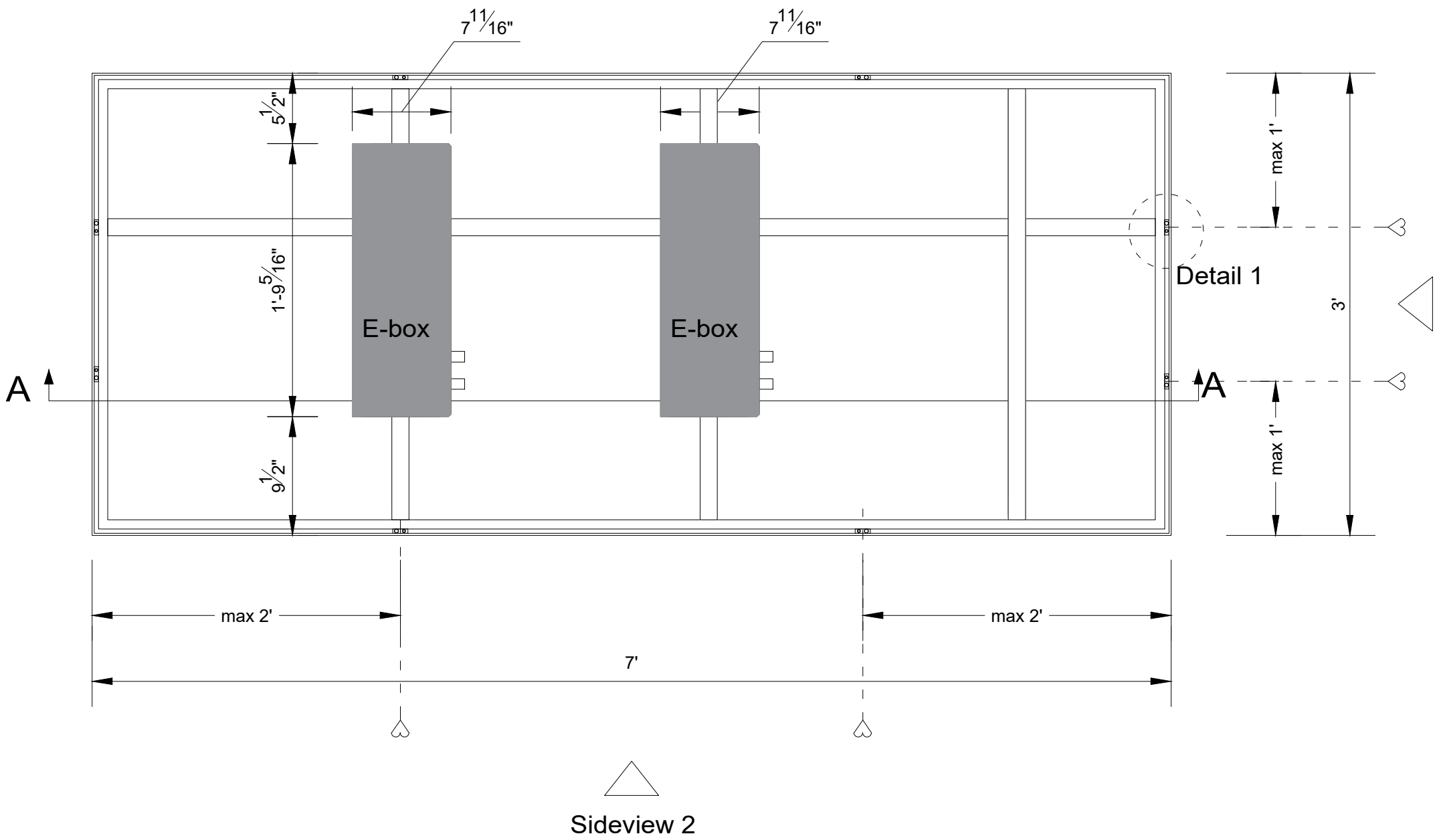
Backview (1:10)
