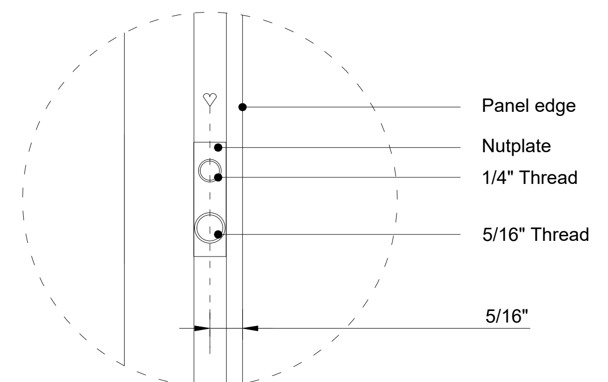
Detail 1 (1:1)
