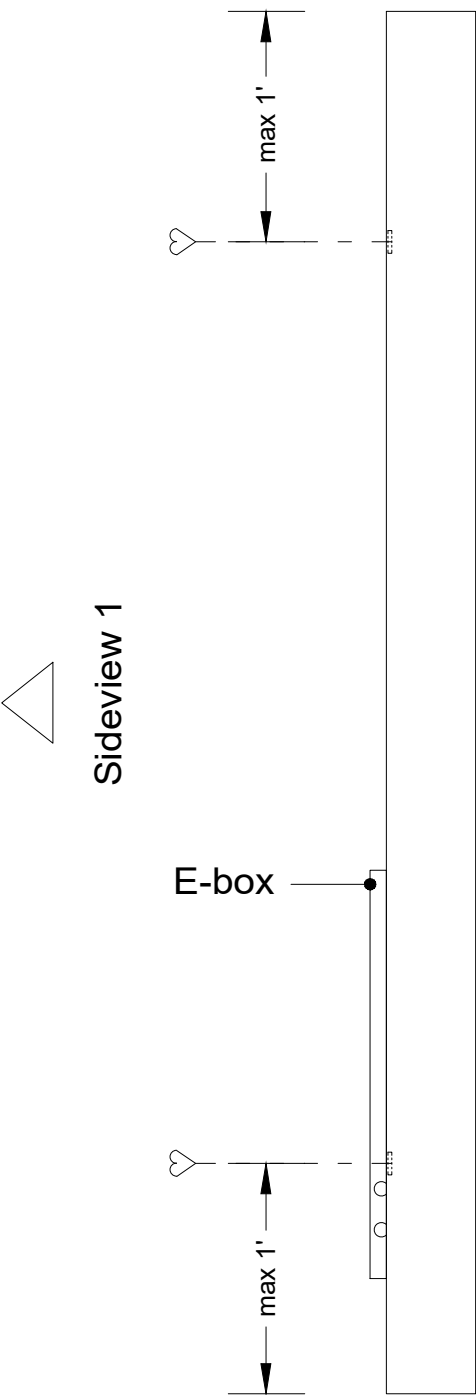
Sideview 1 - mounting position (1:10)
