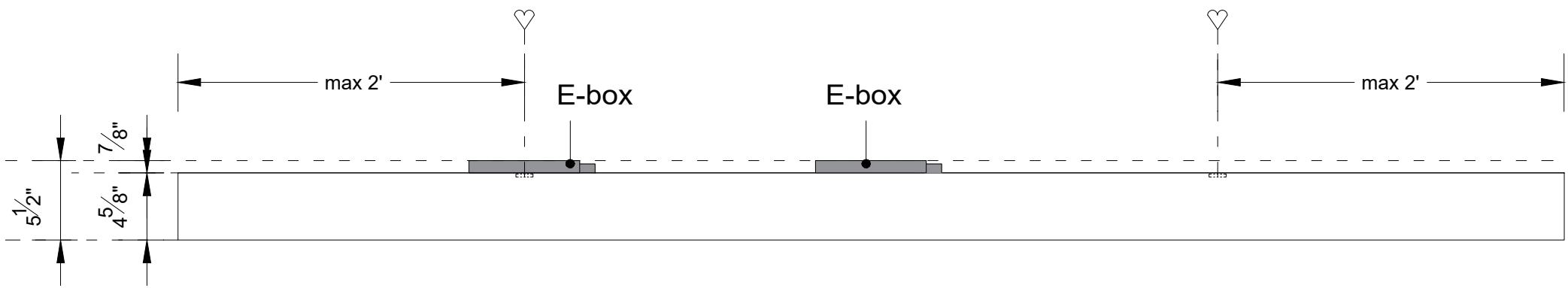
Sideview 2 - mounting position (1:10)
