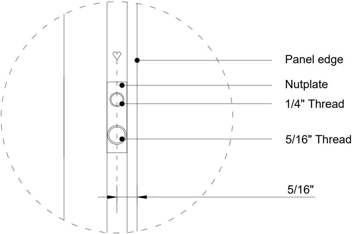
Detail 1 (1:1)
