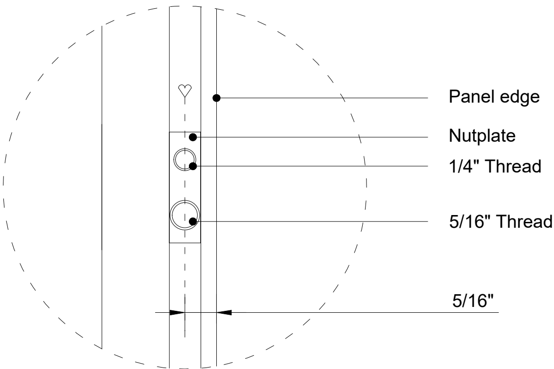
Detail 1 (1:1)
