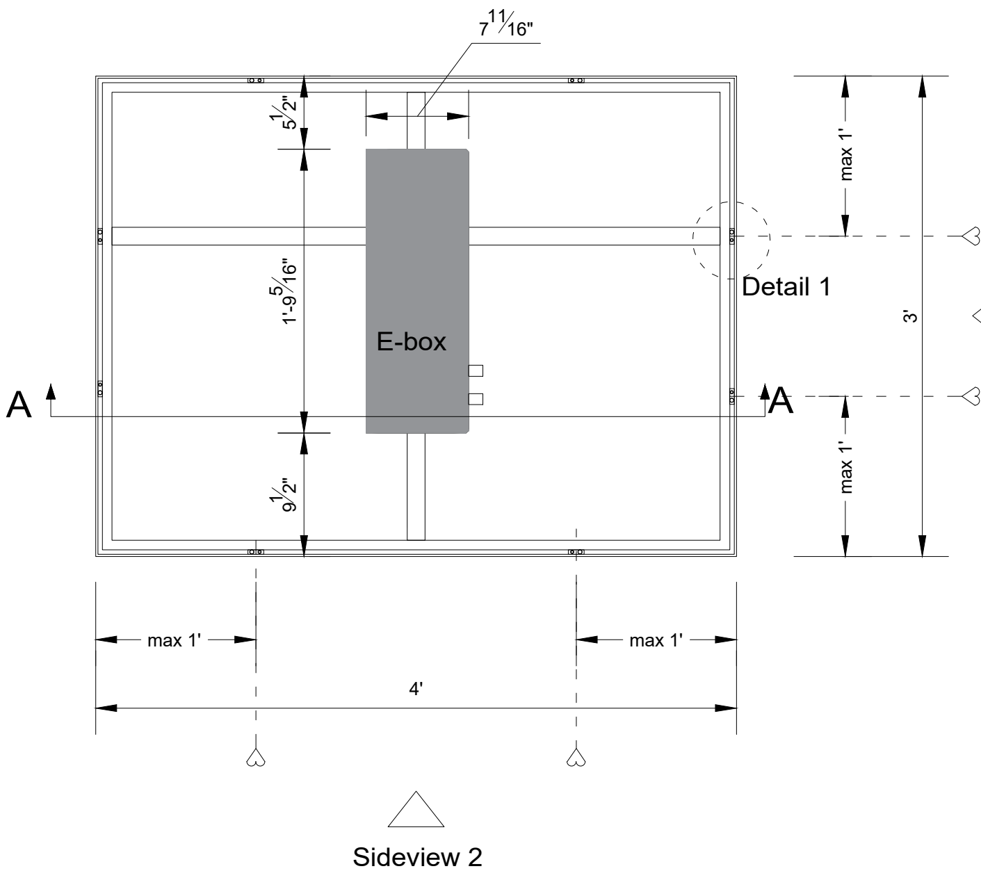
Backview (1:10)
