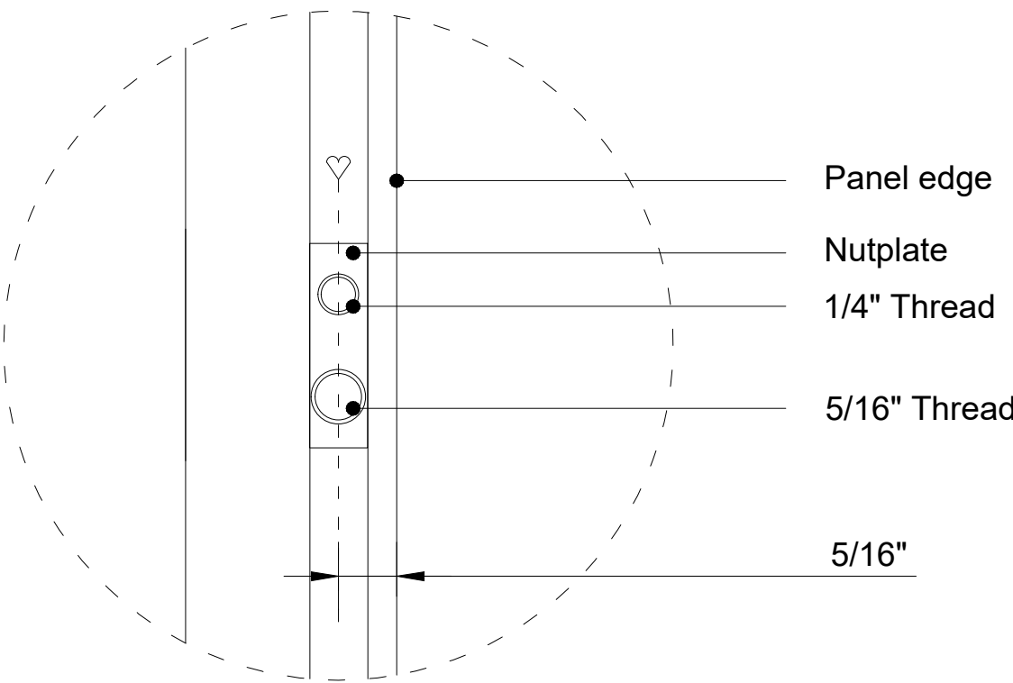
Detail 1 (1:1)
