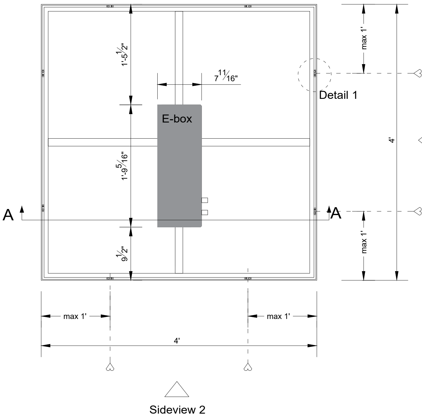
Backview (1:10)
