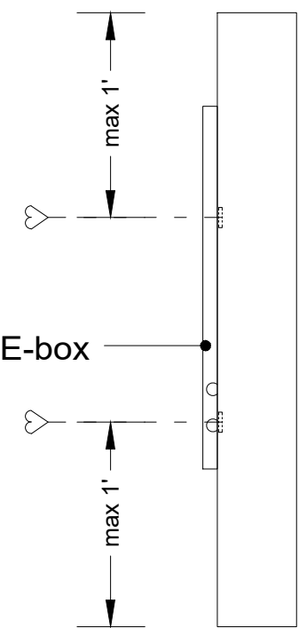
Sideview 1 - mounting position (1:10)
