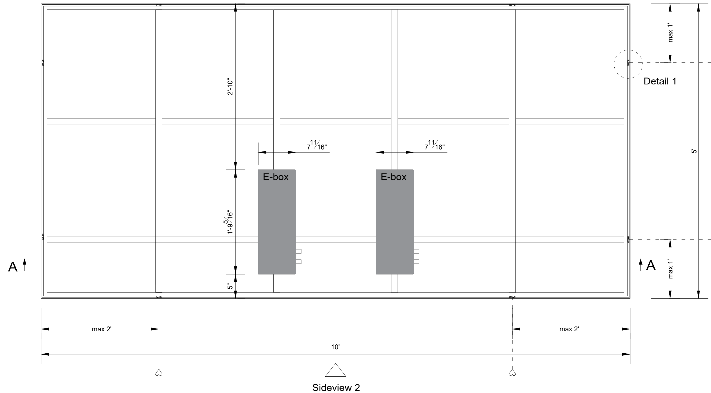
Sideview 2 - mounting position (1:10)
