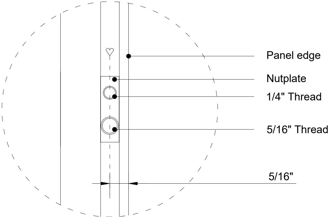
Detail 1 (1:1)
