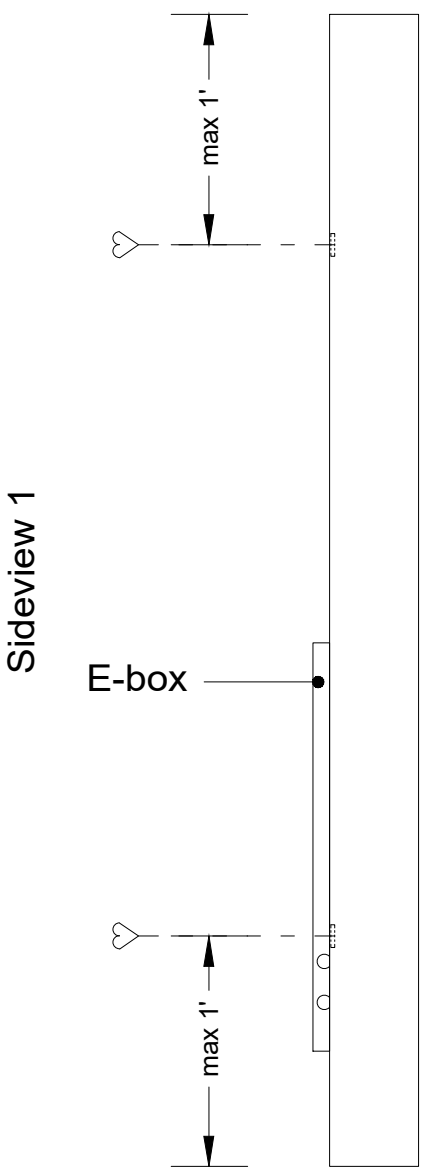
Sideview 1 - mounting position (1:10)
