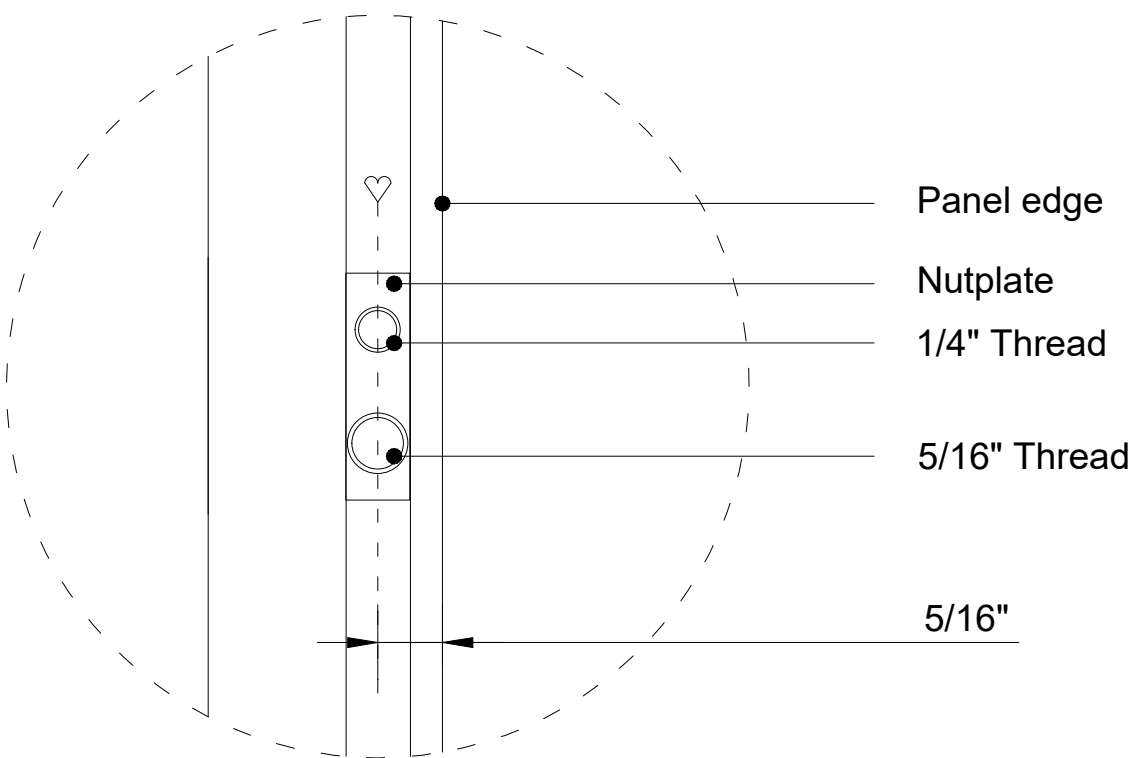
Detail 1 (1:1)
