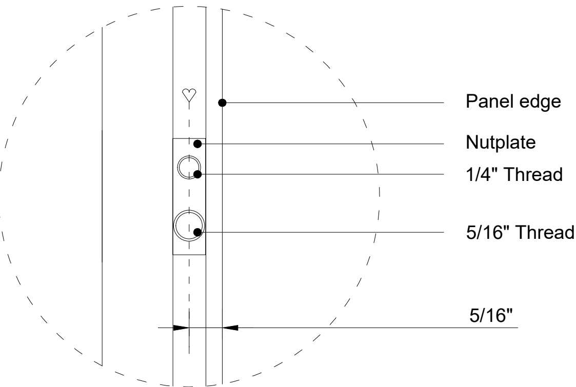
Detail 1 (1:1)
