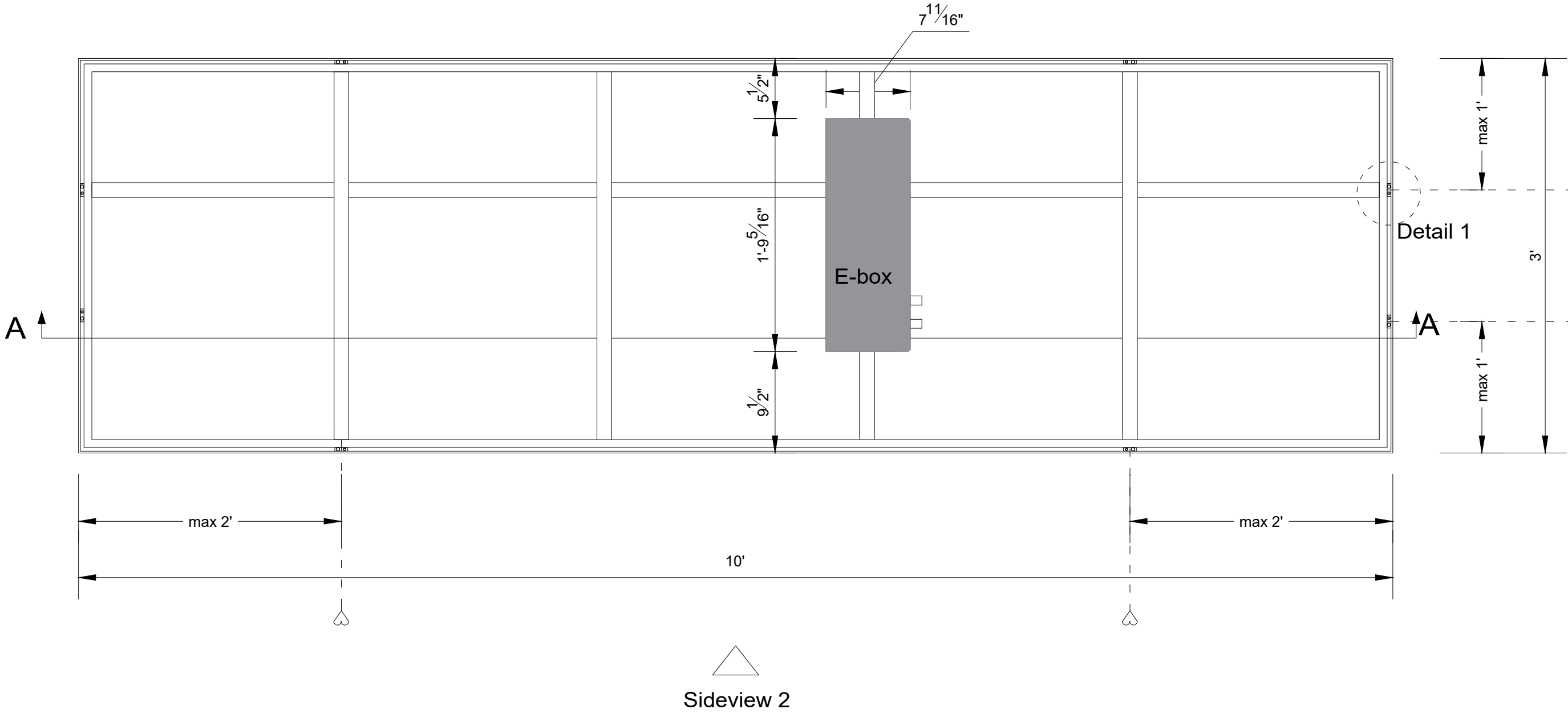
Backview (1:10)
