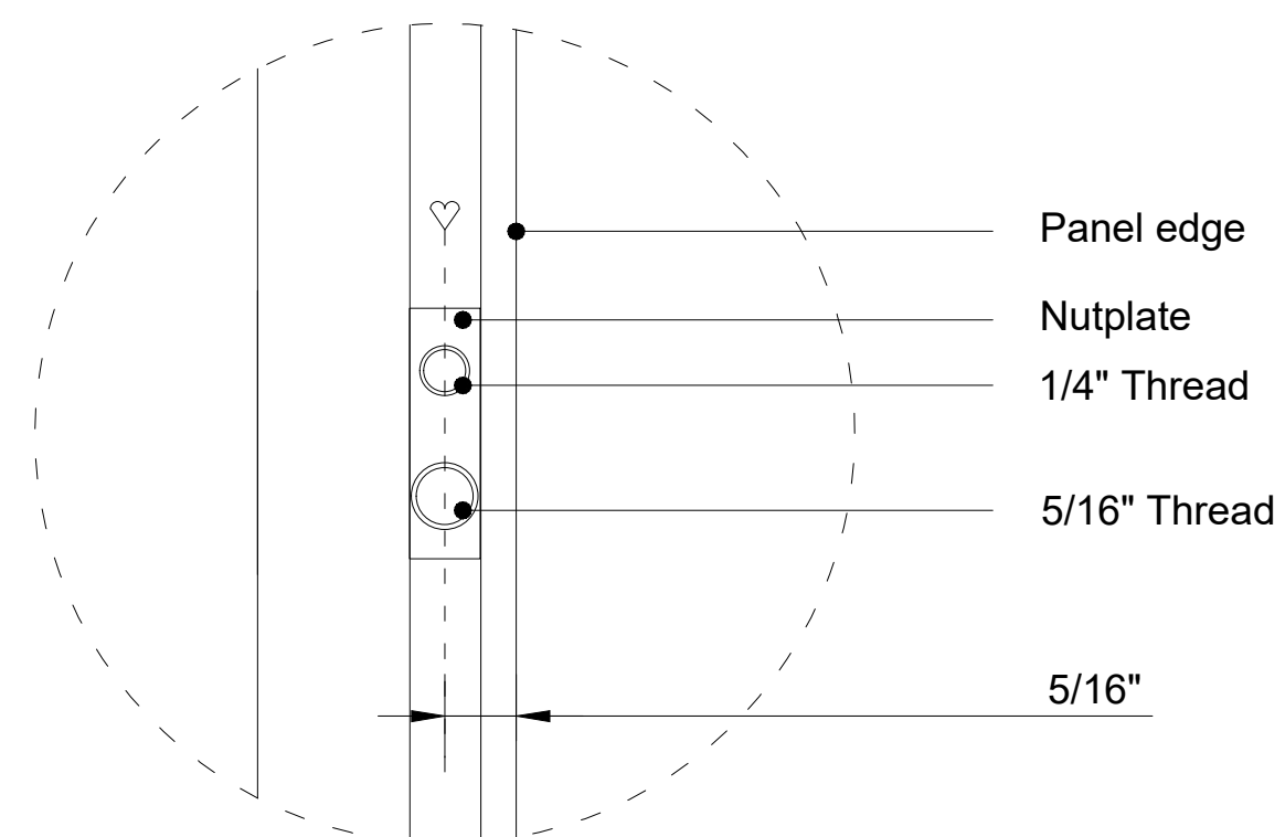
Detail 1 (1:1)
