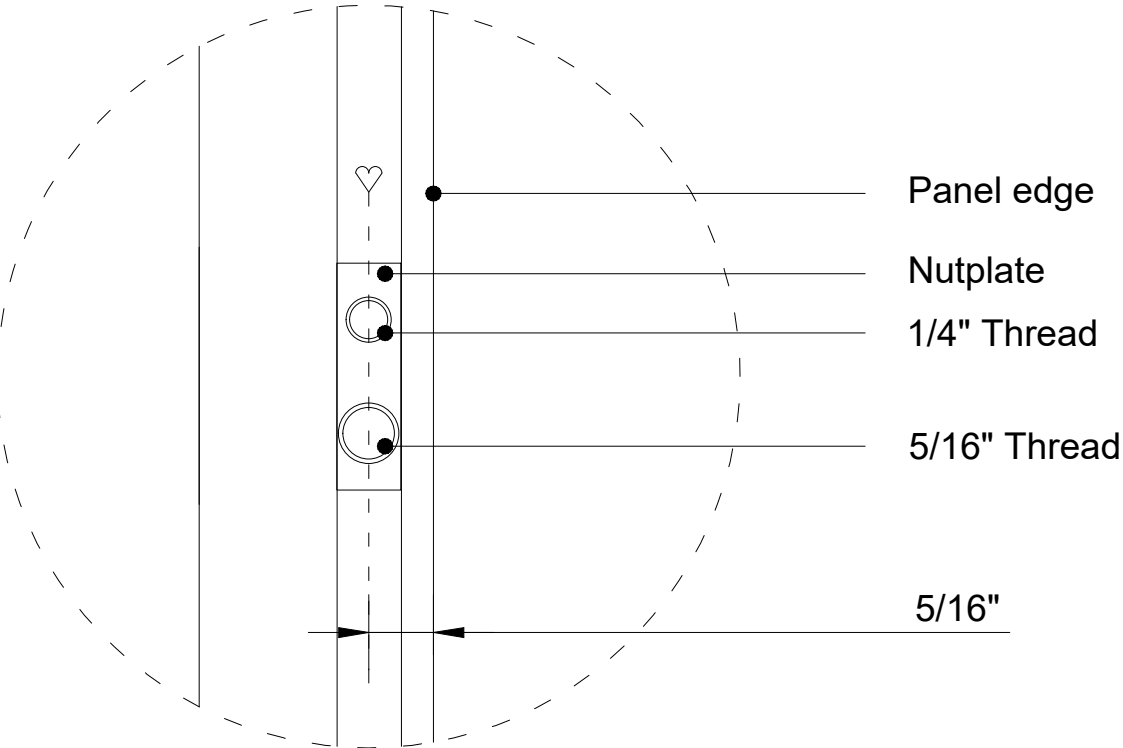
Detail 1 (1:1)
