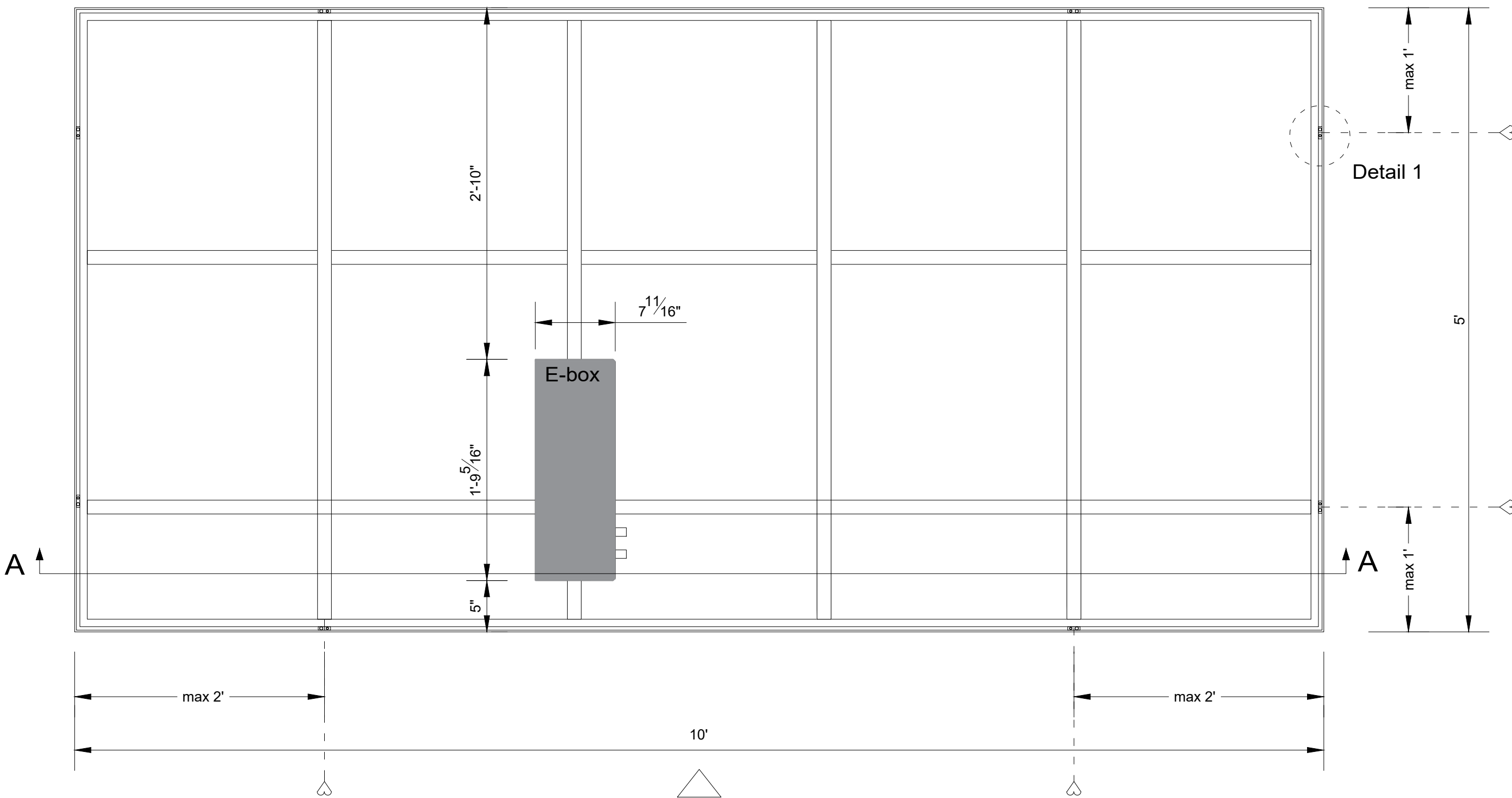
Sideview 2 - mounting position (1:10)
