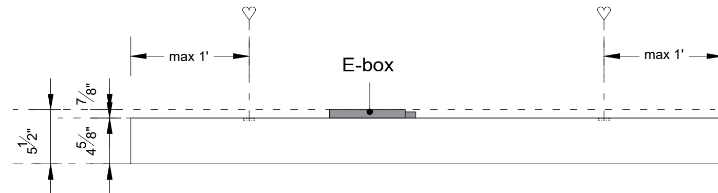
Sideview 2 - mounting position (1:10)
