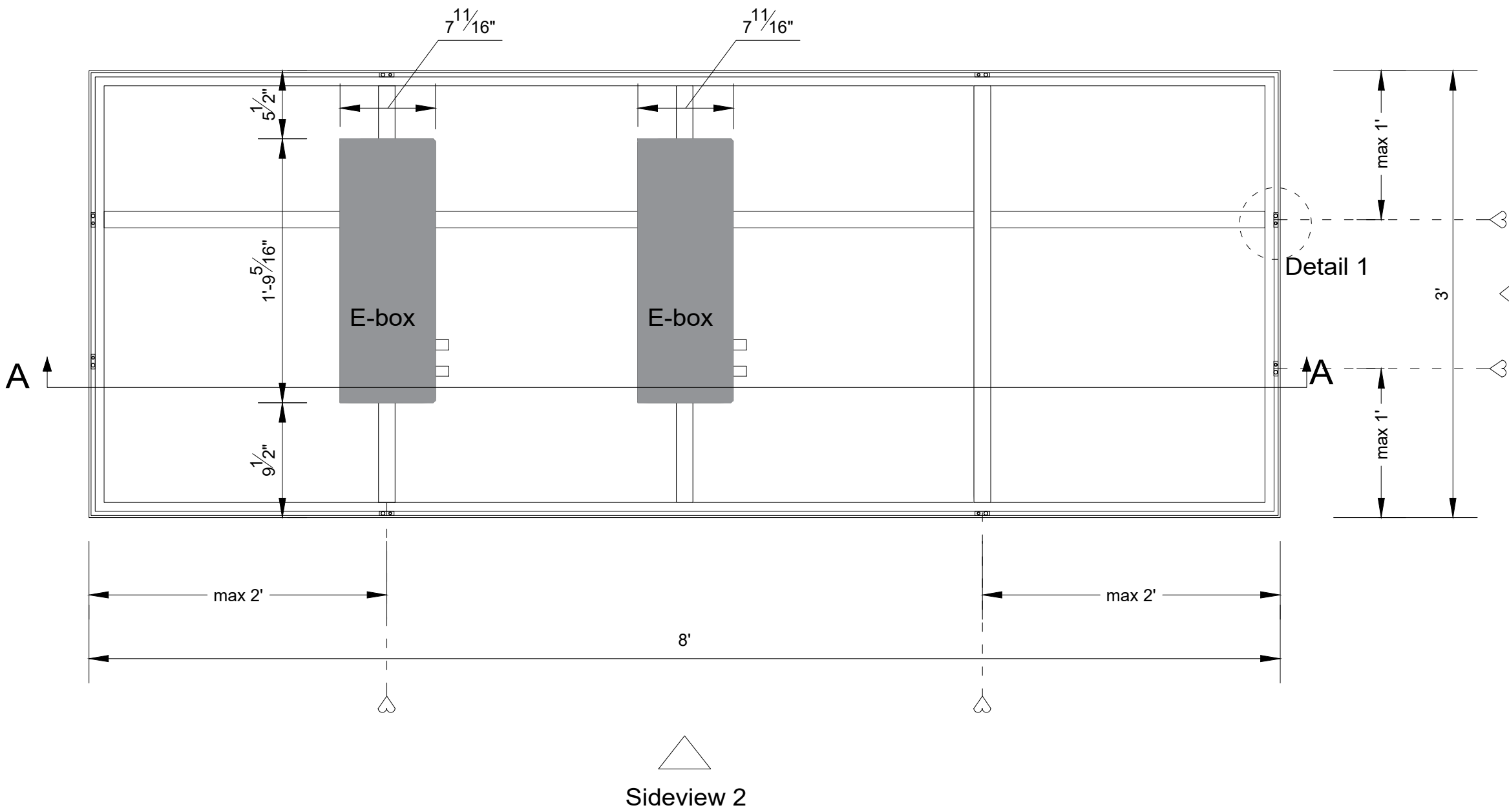
Backview (1:10)
