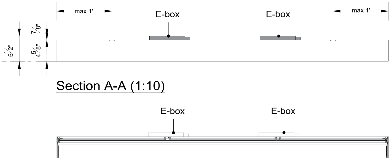
Sideview 2 - mounting position (1:10)
