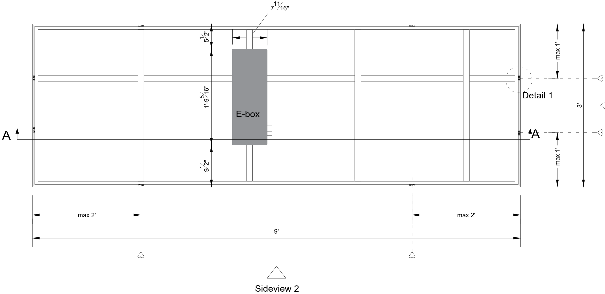
Backview (1:10)
