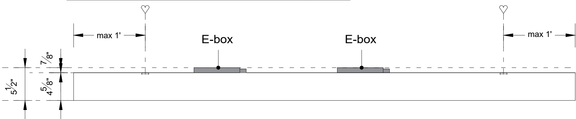
Section A-A (1:10)
