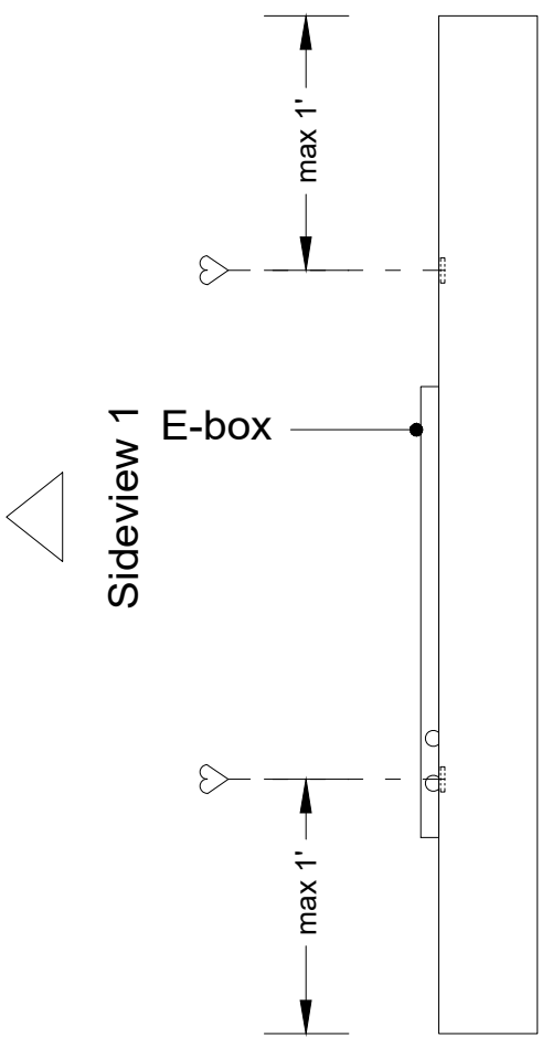
Sideview 1 - mounting position (1:10)
