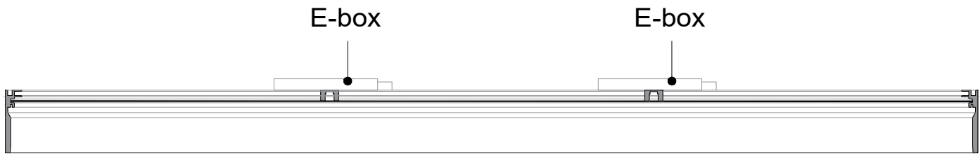
Section A-A (1:10)
