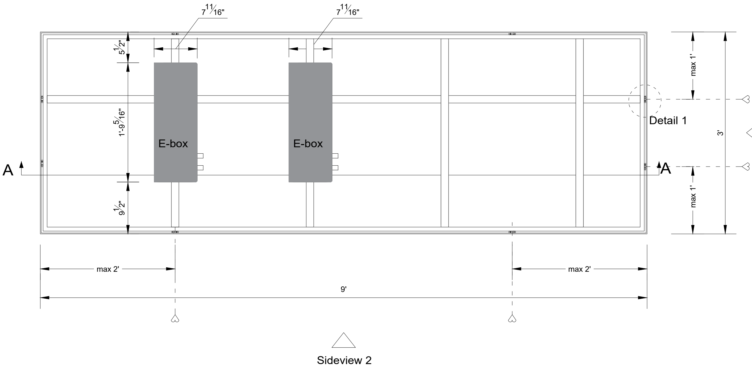
Backview (1:10)
