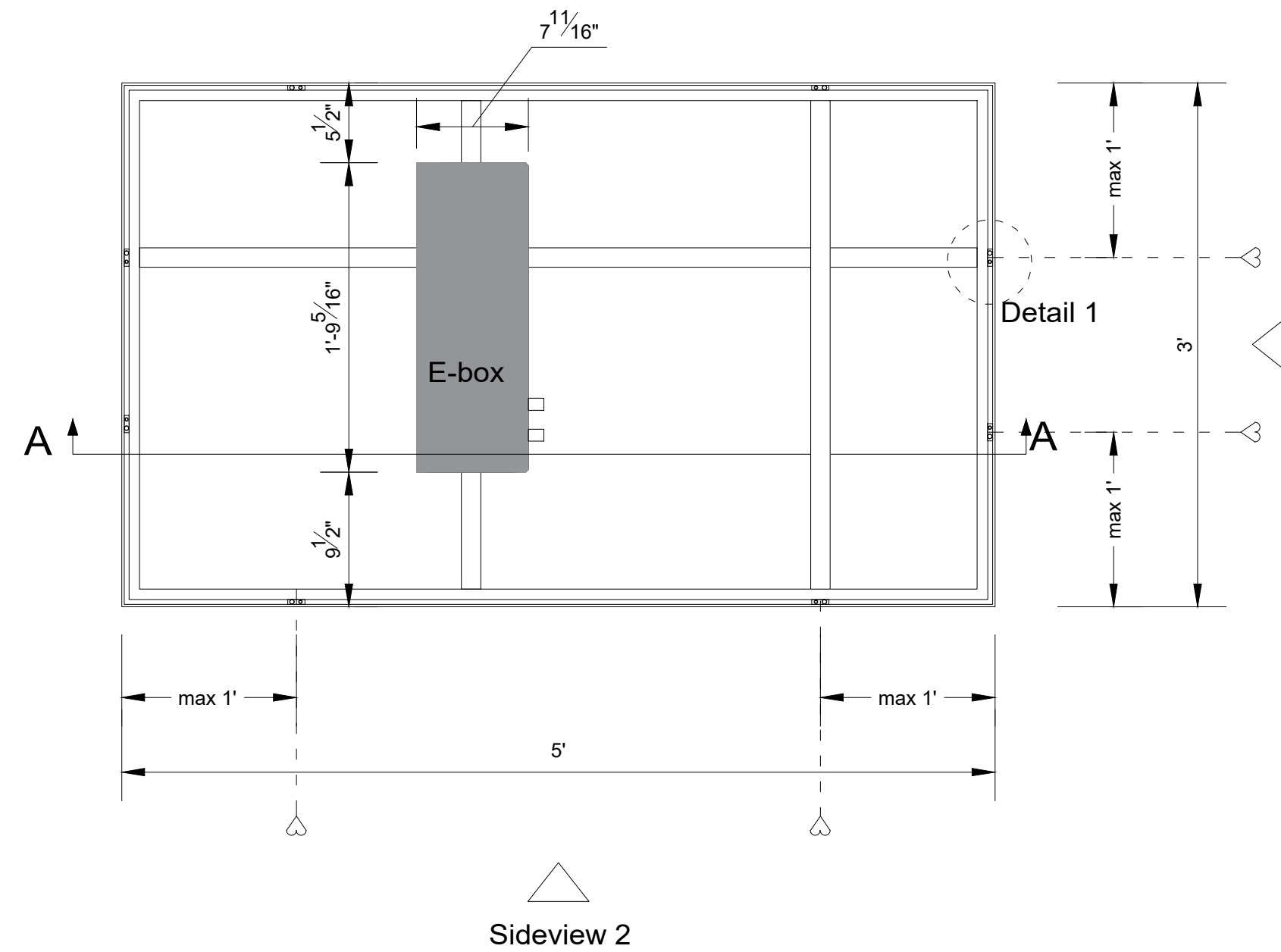
Backview (1:10)
