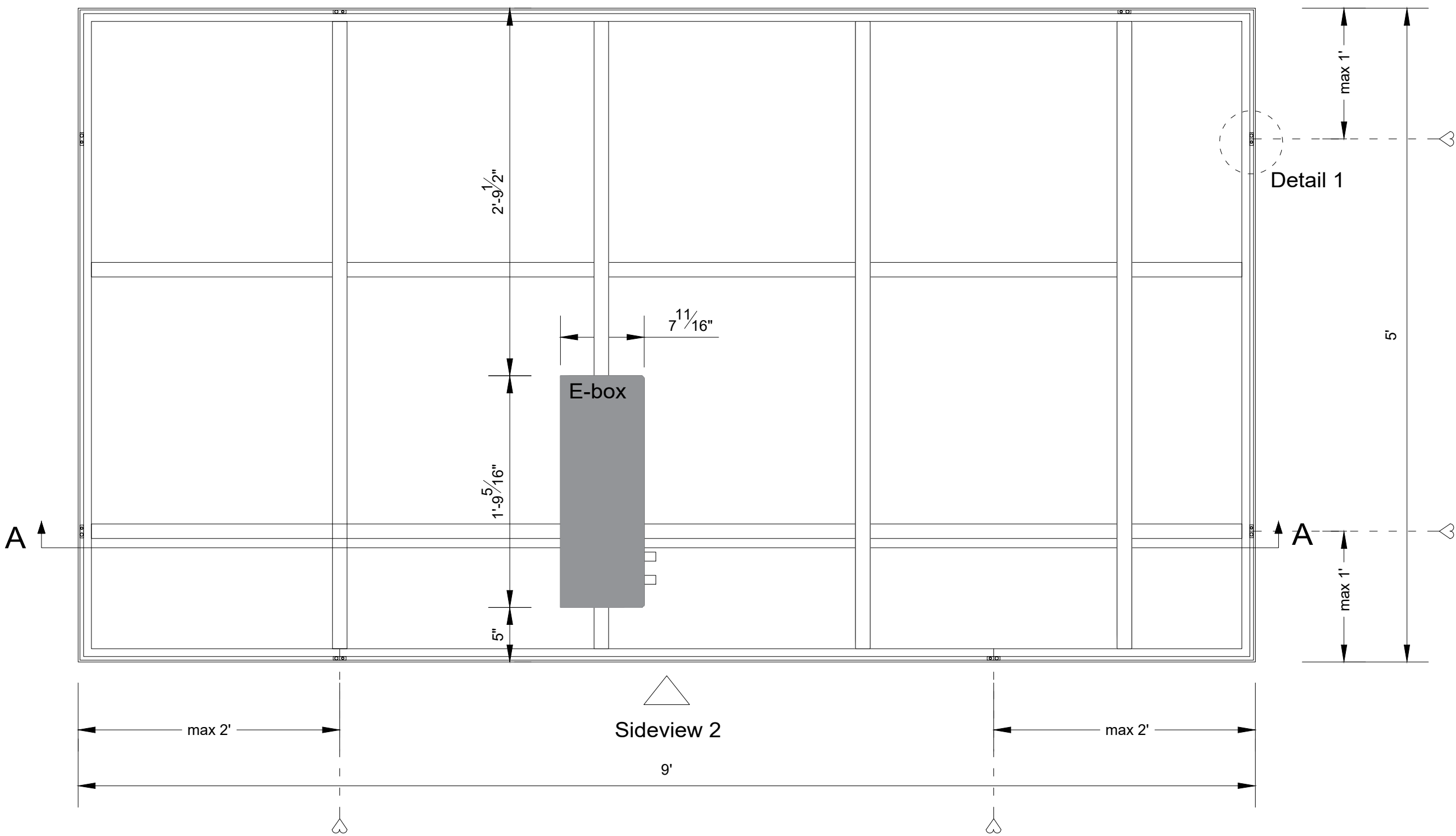
Sideview 2 - mounting position (1:10)
