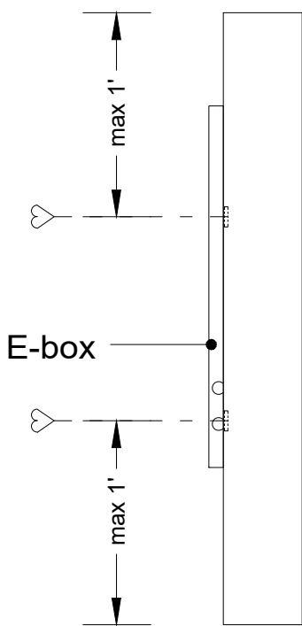
Sideview 1 - mounting position (1:10)
