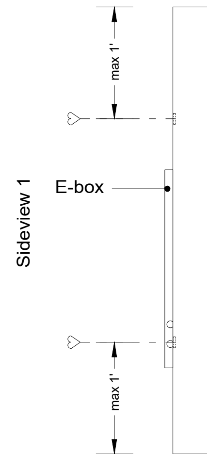
Sideview 1 - mounting position (1:10)
