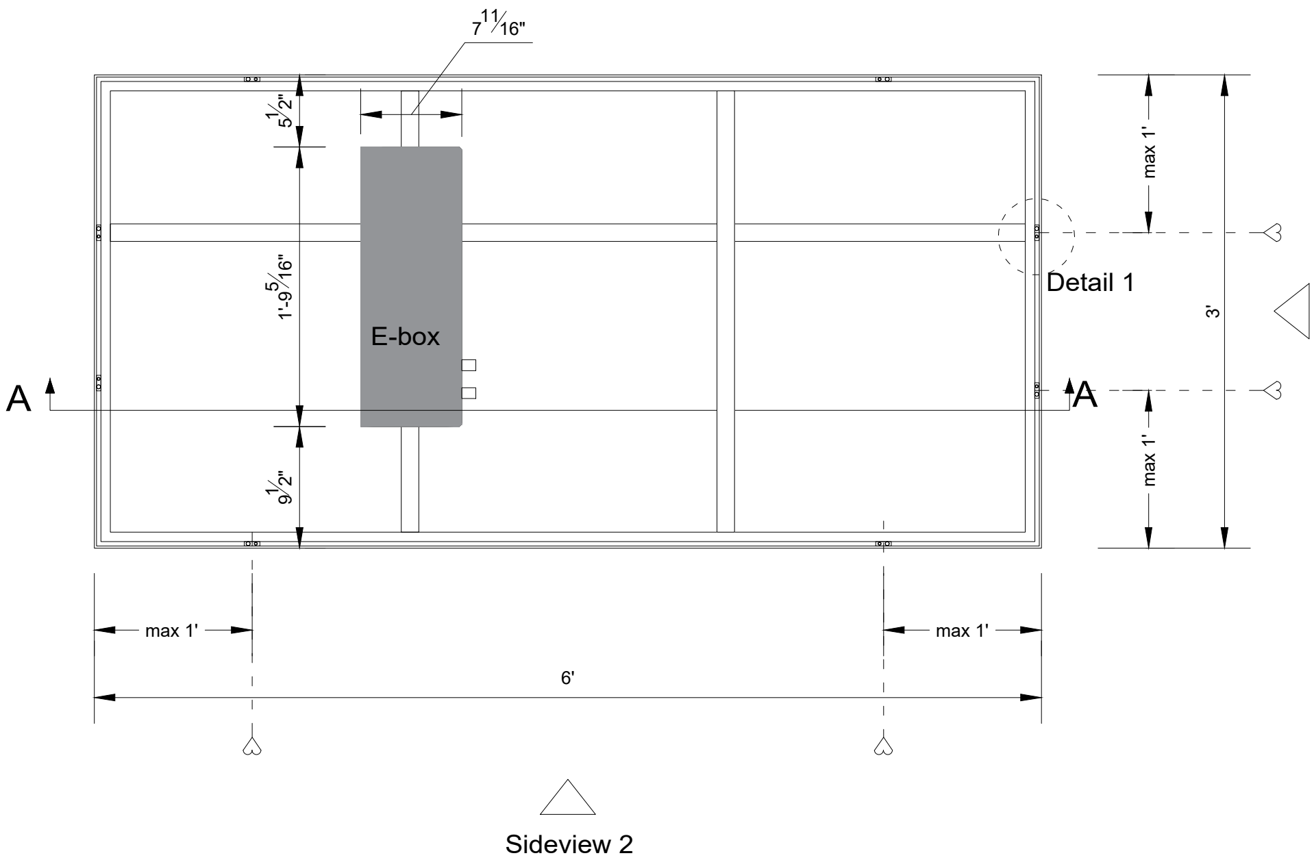
Backview (1:10)
