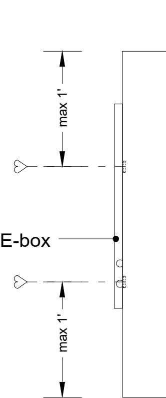
Sideview 1 - mounting position (1:10)
