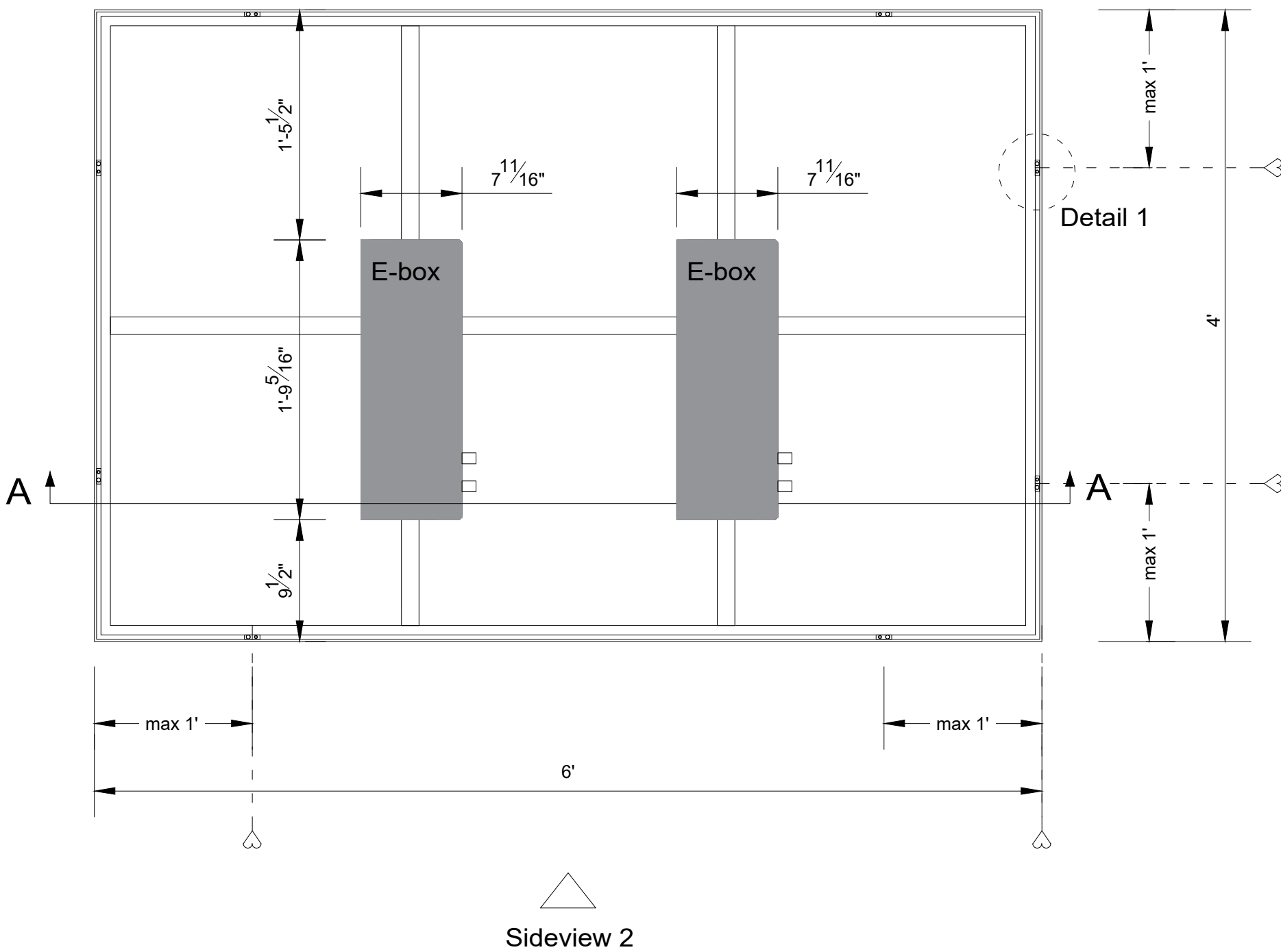
Backview (1:10)
