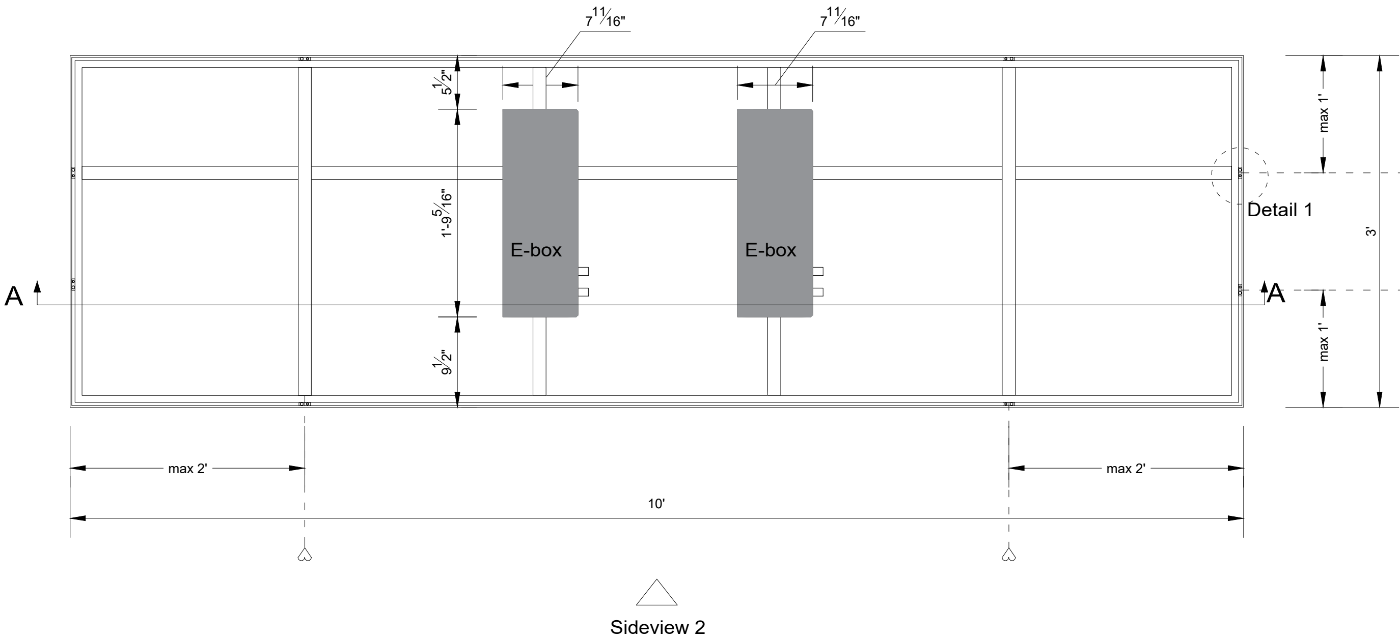
Backview (1:10)
