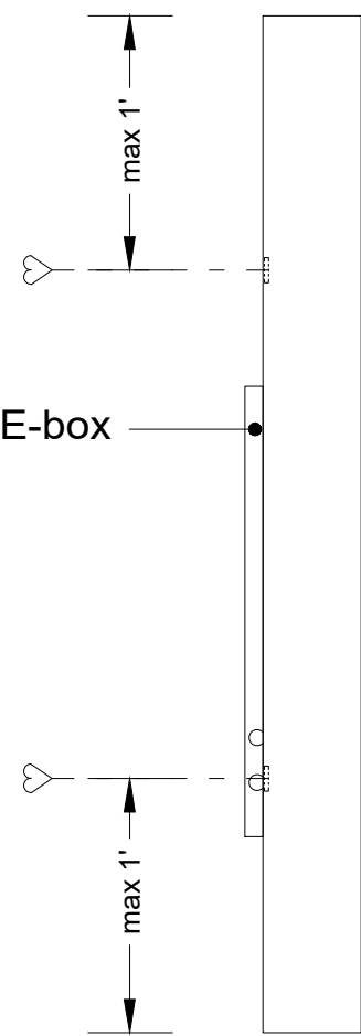
Sideview 1 - mounting position (1:10)
