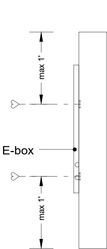
Sideview 1 - mounting position (1:10)
