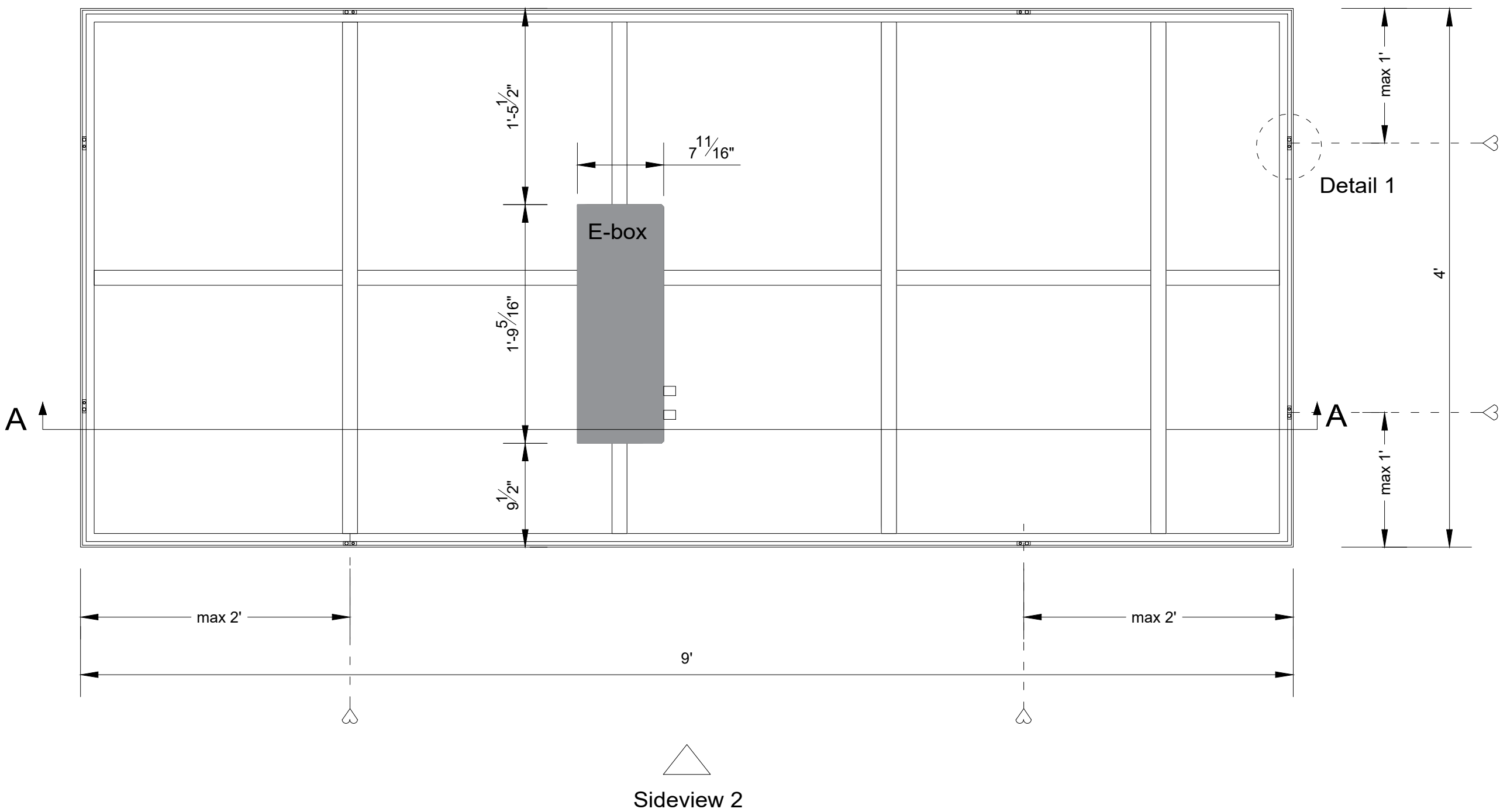
Backview (1:10)
