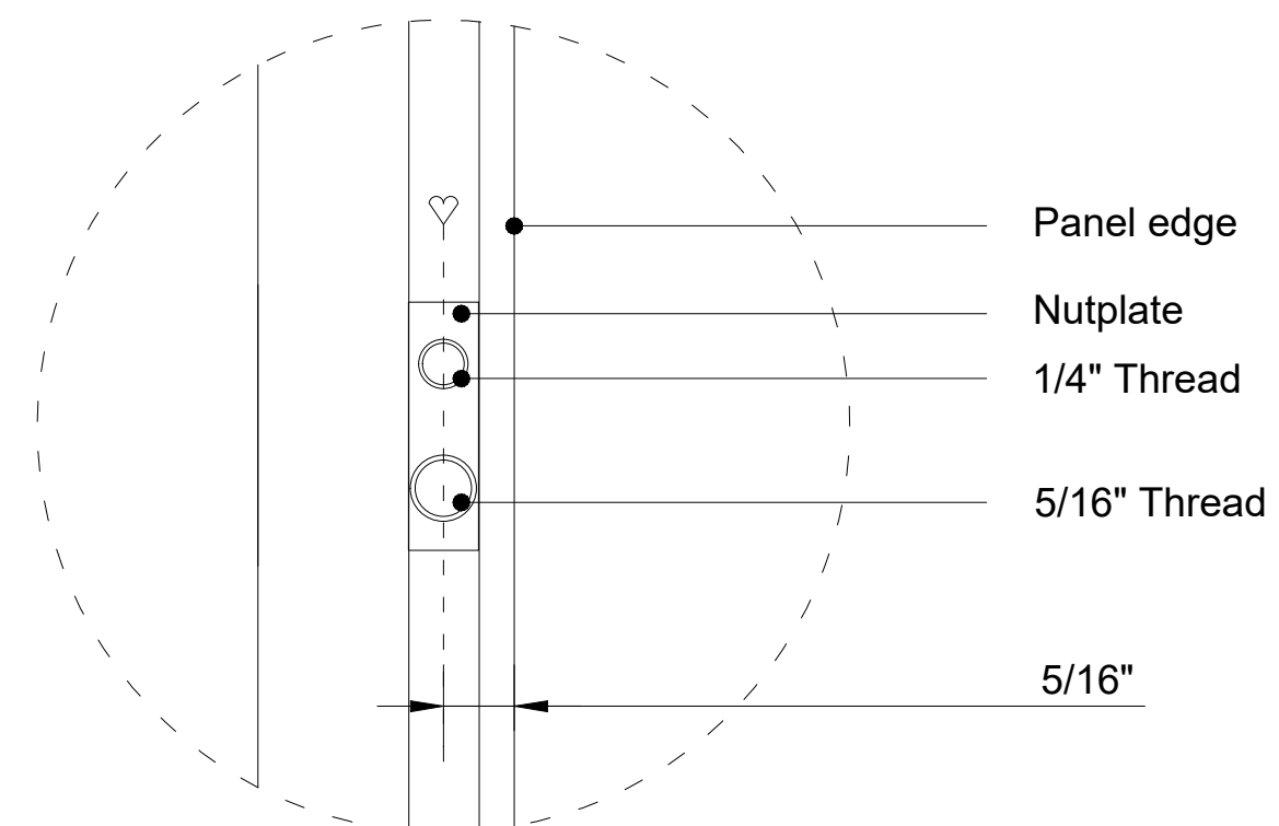
Detail 1 (1:1)
