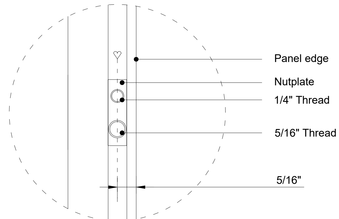
Detail 1 (1:1)
