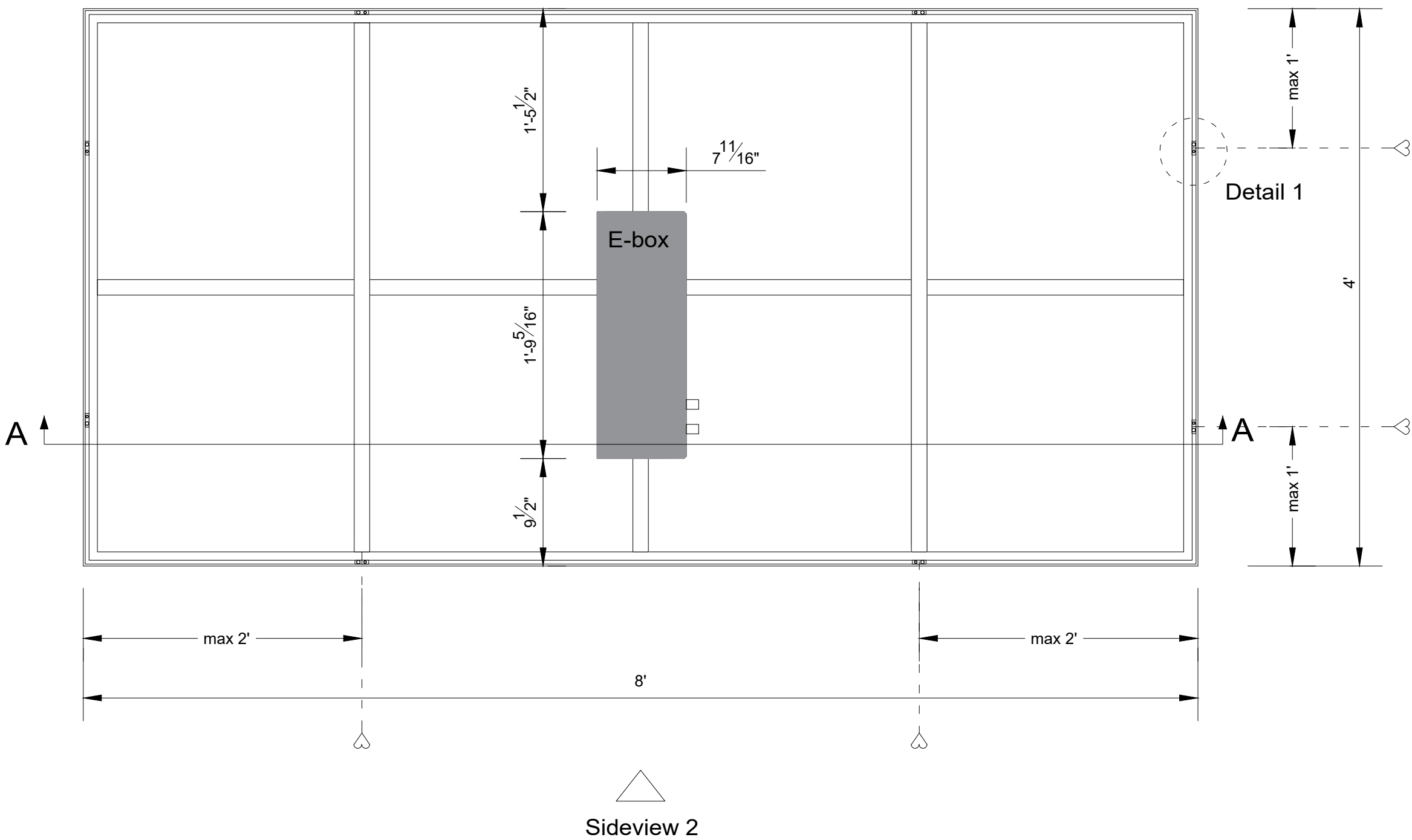
Backview (1:10)
