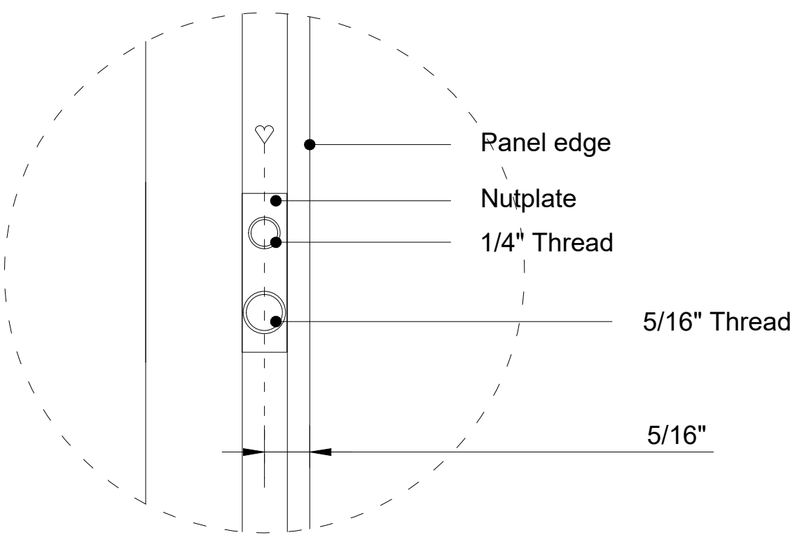
Detail 1 (1:1)
