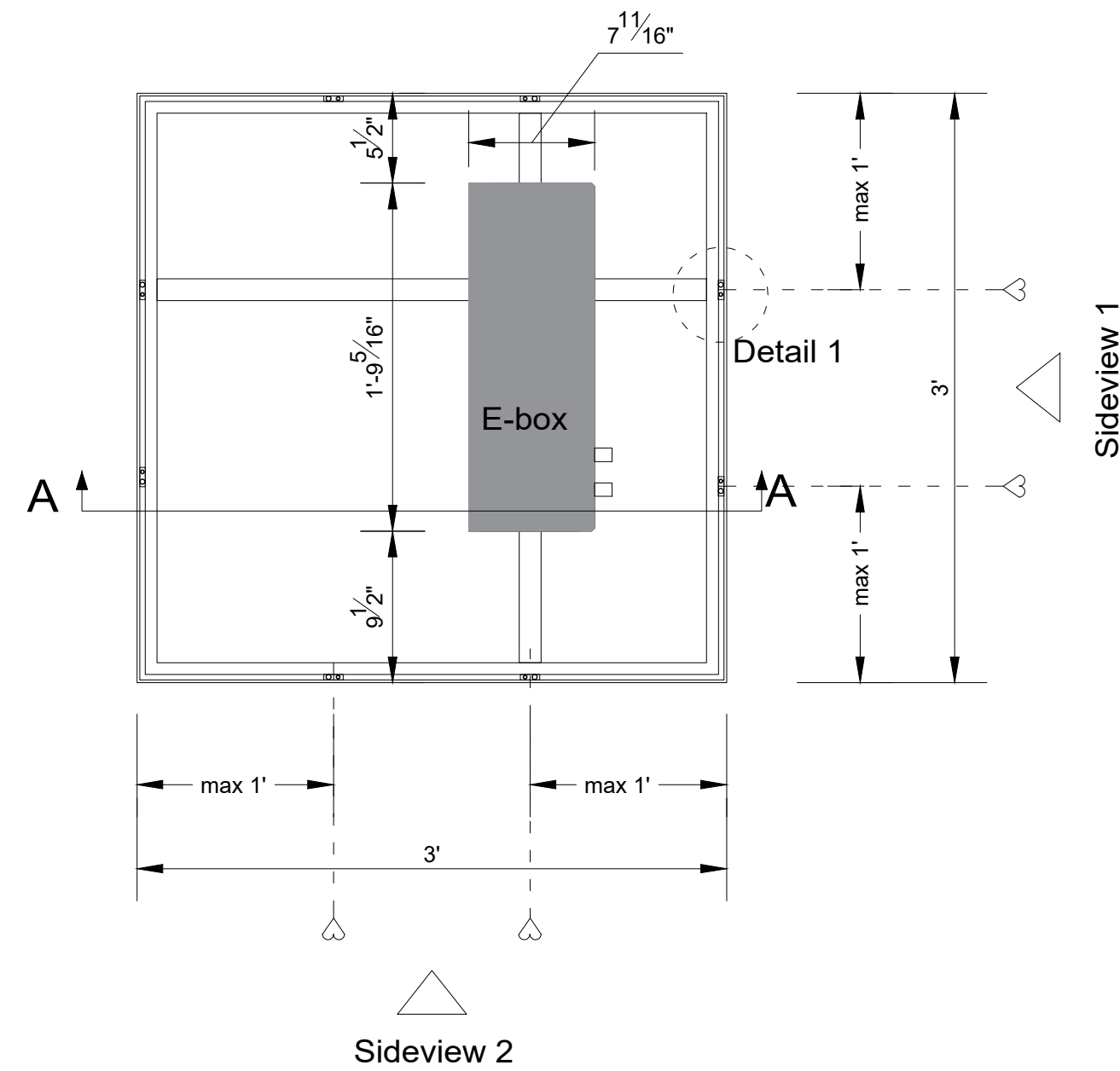
Backview (1:10)
