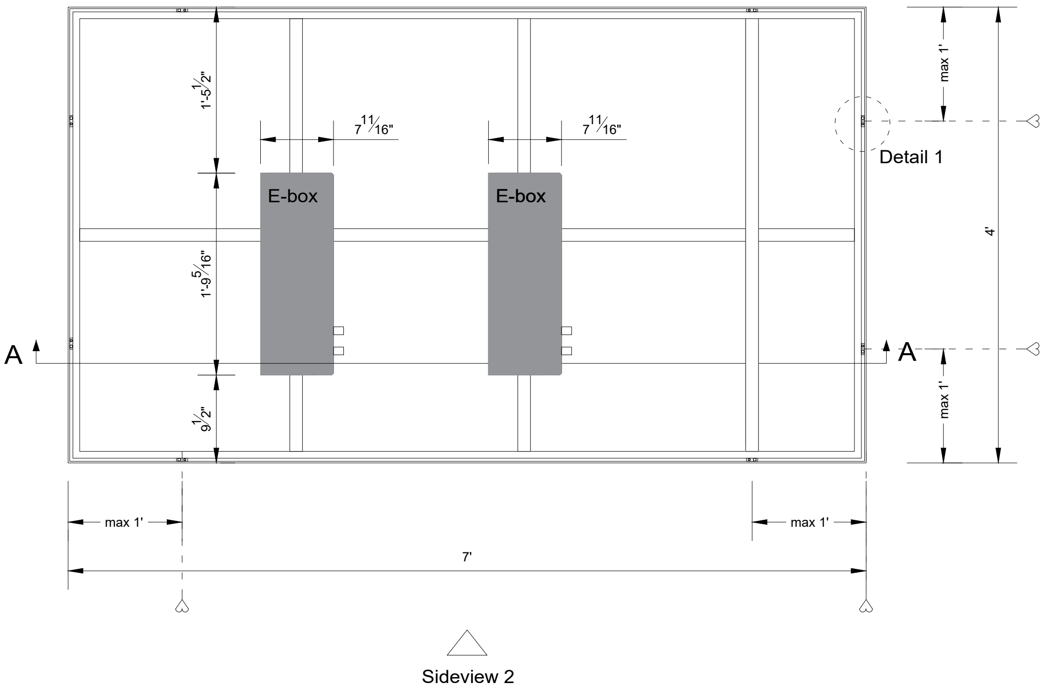
Backview (1:10)
