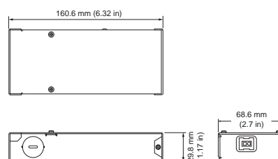
Cove QLX Wiring Compartment
