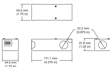
Cove MX Wiring Compartment
