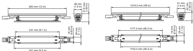
eW Cove MX, 125° x 120°
