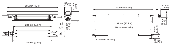
eW Cove MX, 50° x 70°
